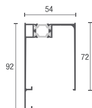
code 4585 Upper and side profile TT in AL
