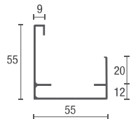
code 4047 Base AL profile
