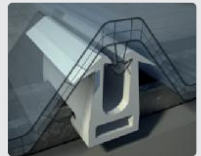
ANCHORAGE OF ROOFING This is done by pressing onto the anchor bracket.
