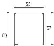
code 4045 Upper and side AL profile
