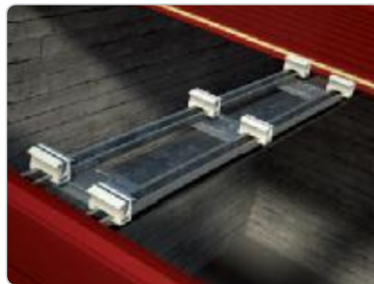
OVERLAP - STEP 1 Detail of double anchor bracket anchored to roofing structure
