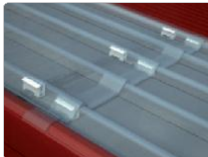
OVERLAP - STEP 3 Insertion of upper sheet by pressing
