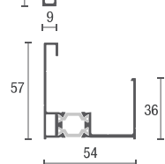
code 4587 Base profile TT in AL
