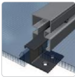
SYSTEM WITH ALUMINIUM CONNECTOR CODE 4310
