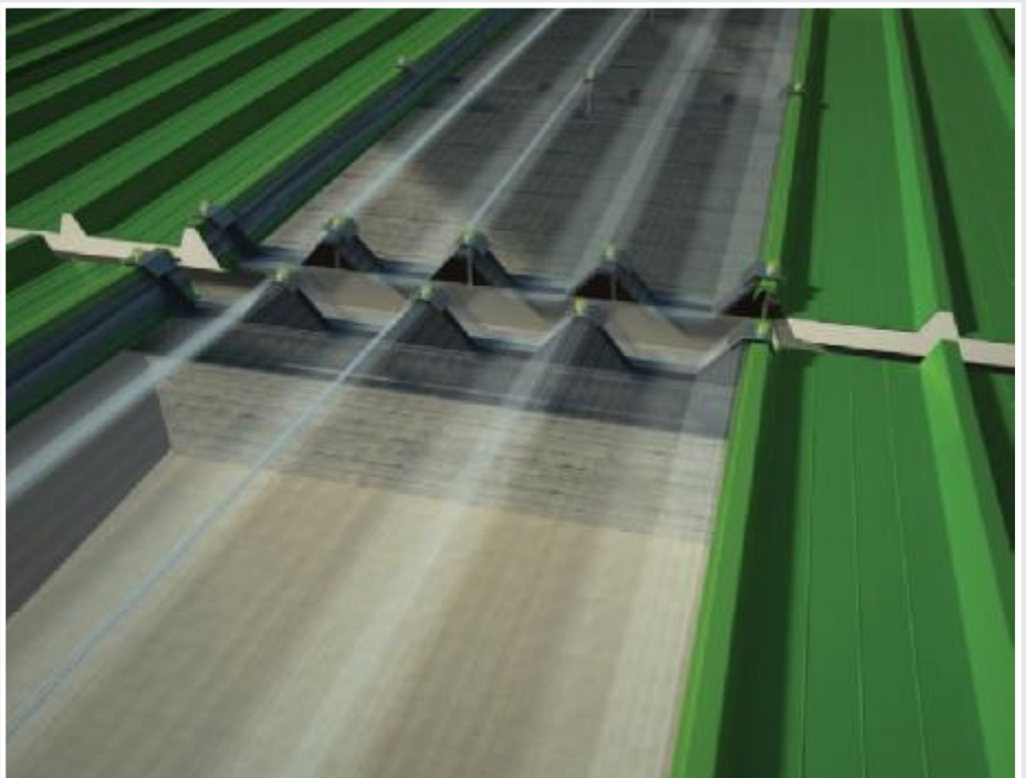
SKYLIGHT - PANEL APPLICATION Construction of skylight with lateral overlapping of insulating roofing panels. Detail of valley gutter.
