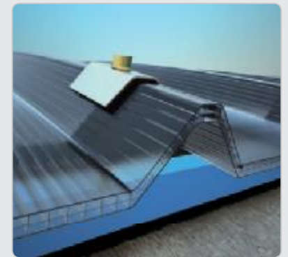
ANCHORAGE OF ROOFING This is done by drilling and inserting a screw with Vipla washer and cap.
