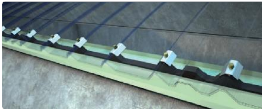
DETAIL OF OVERLAP Detail of double anchor bracket anchored to roofing structure
