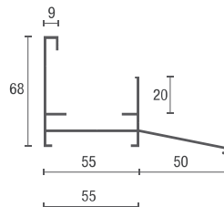
code 4046 Base AL profile with eave
