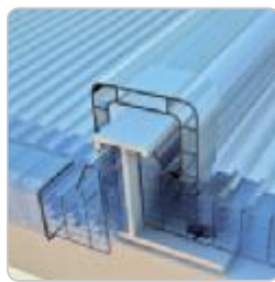
SYSTEM WITH POLYCARBONATE COVERGASKET CODE 2146
