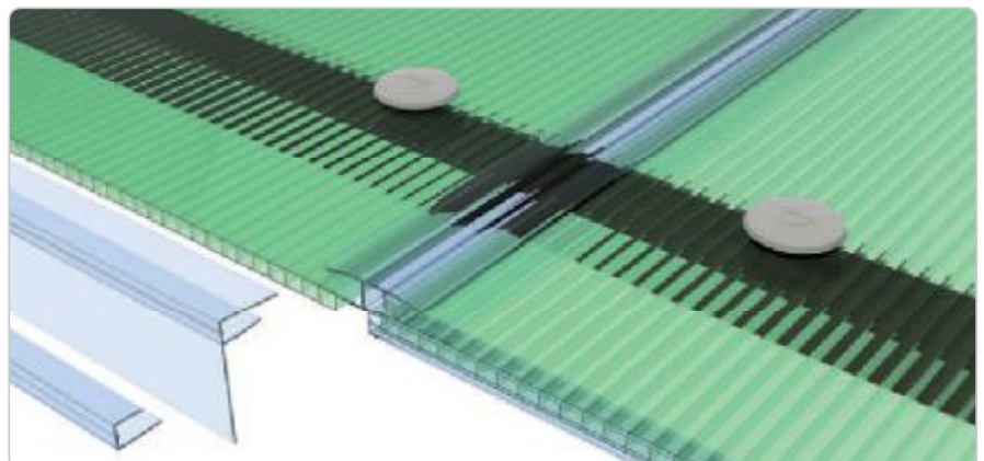
CONTINUOUS ROOFING Detail of roof with H-shaped connector and air cell end profiles.
